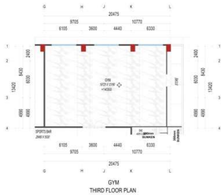
GYM – PART PLAN
