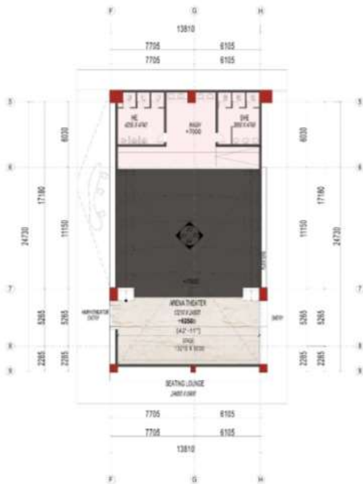
ARENA THEATRE – PART PLAN
