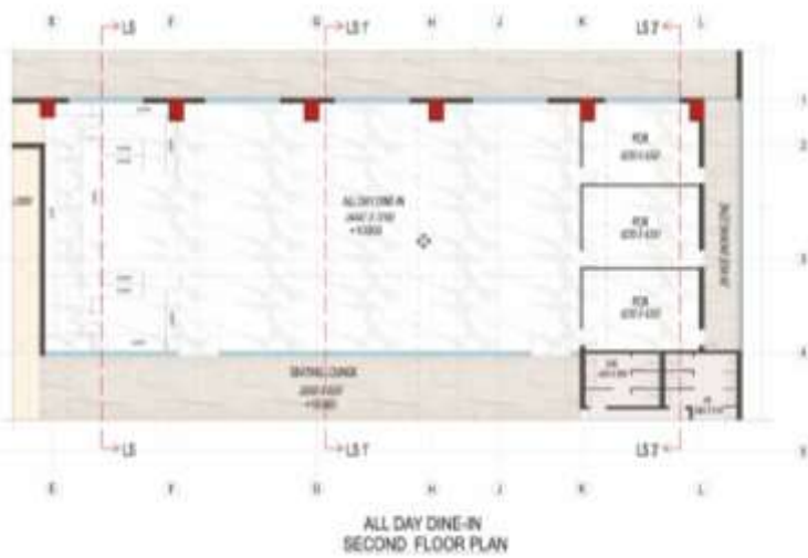
ALL DAY DINING – PART PLAN
